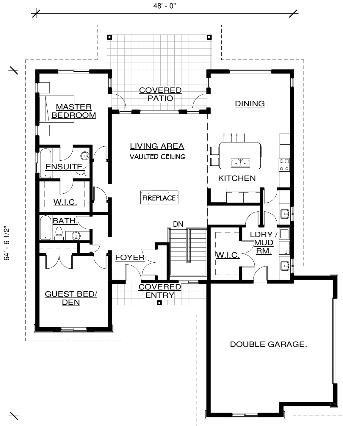
Main Floor Plan 3/32" = 1'-0"
