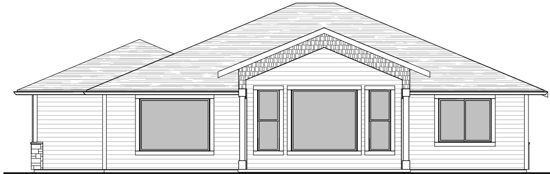
Rear Elevation \frac{3}{32}'' = 1'-0''
